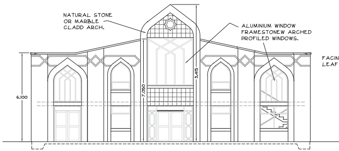
PROPOSED FRONT ELEVATION FACING TONTINE ST. (NORTHWEST ELEVATION).
