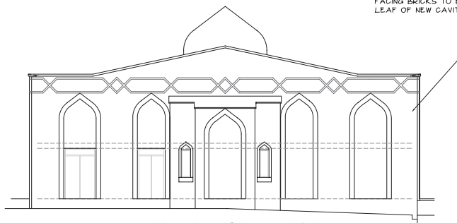
PROPOSED REAR GABLE ELEVATION. (SOUTHEAST ELEVATION).
